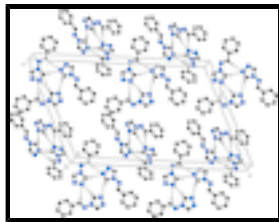
Fig. 2. The crystal packing of the title compound, showing the formation of hydrogen-bonded (dashed lines) trimers.
